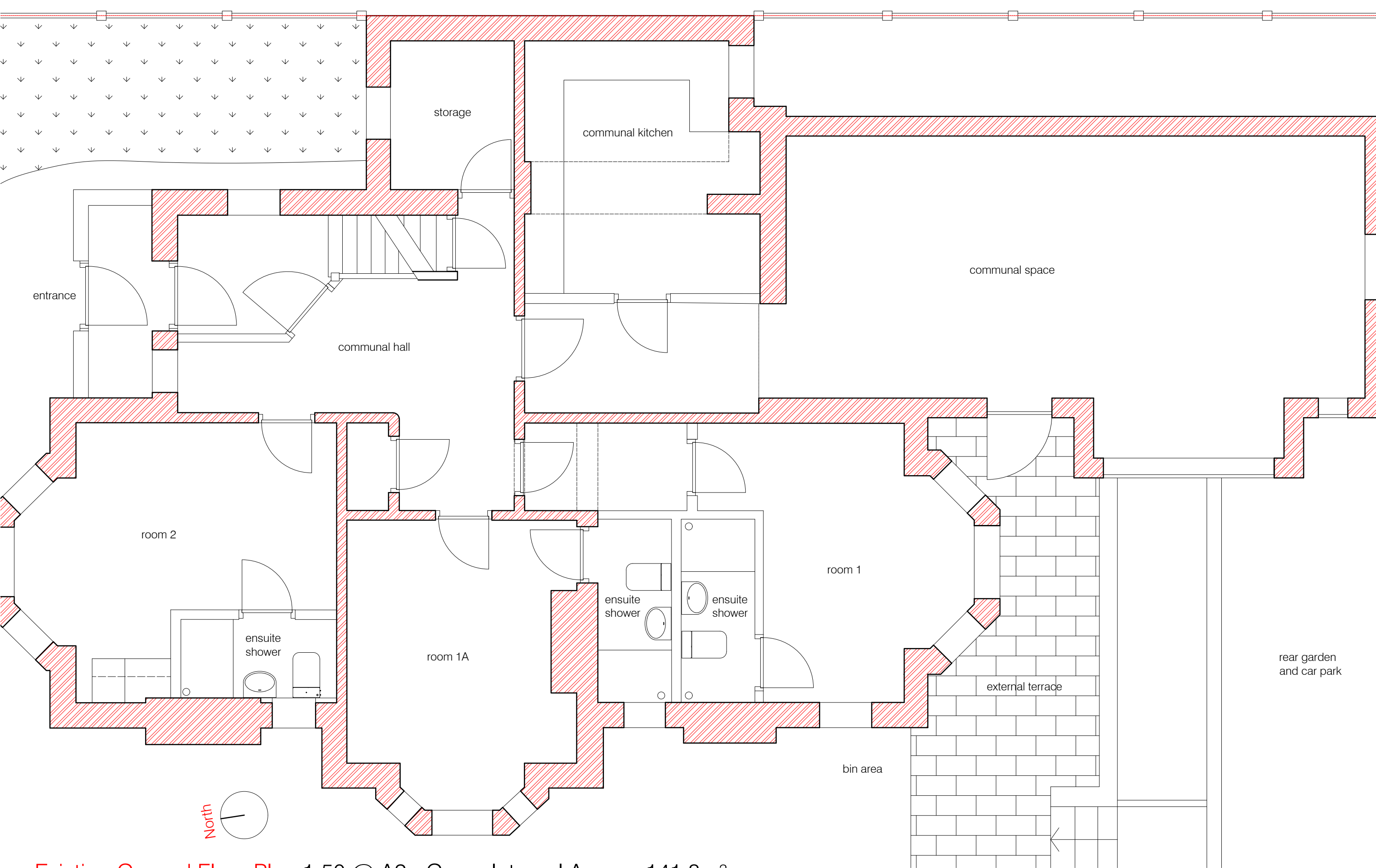
Existing Ground Floor Plan 1:50 @ A2 - Gross Internal Area = 141.8m 2
