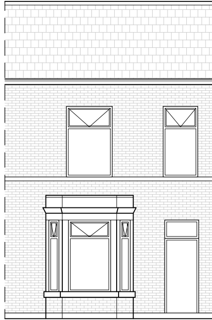
EXISTING FRONT ELEVATION 1:100 @ A3
