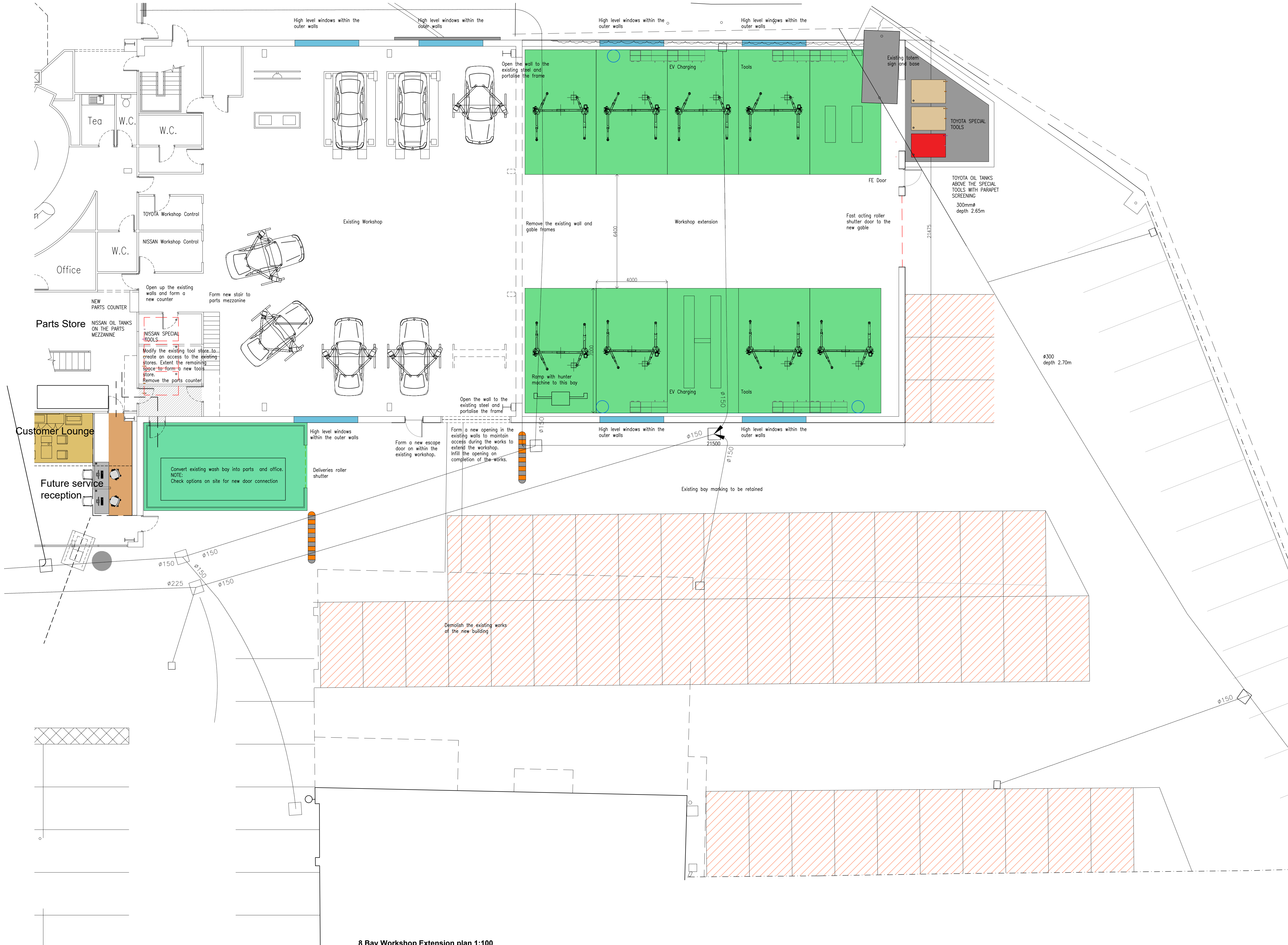
8 Bay Workshop Extension plan 1:100
