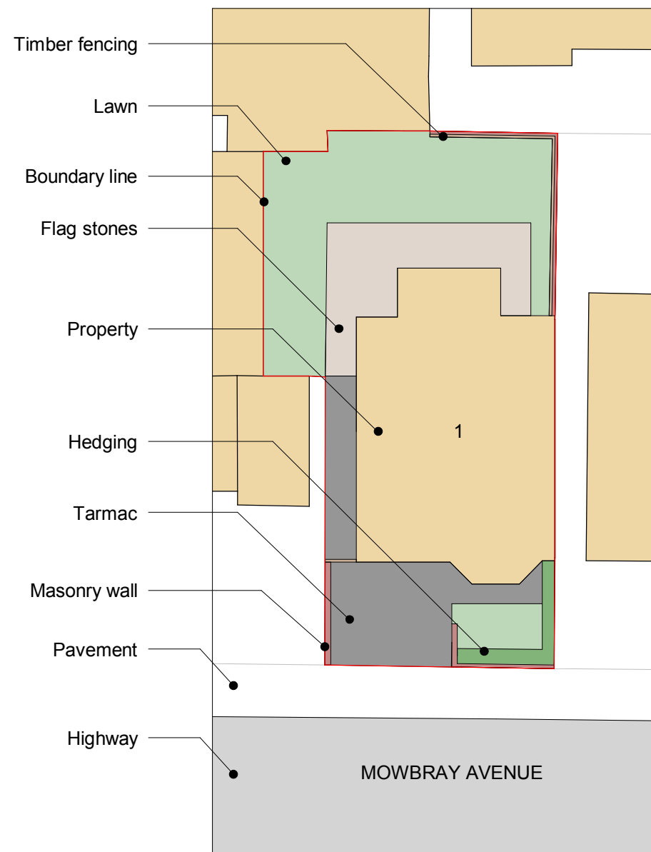
1. Site Layout - Existing
