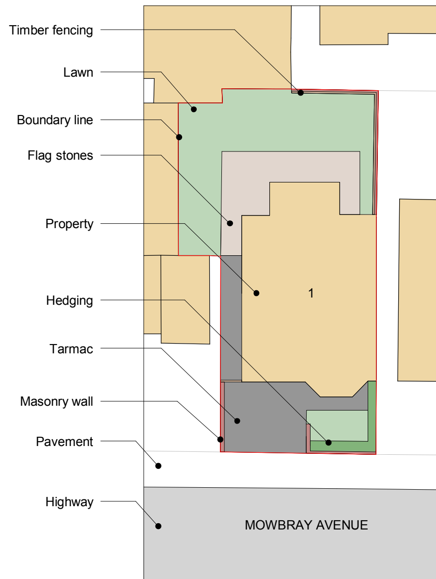
2. Site Layout - Proposed
