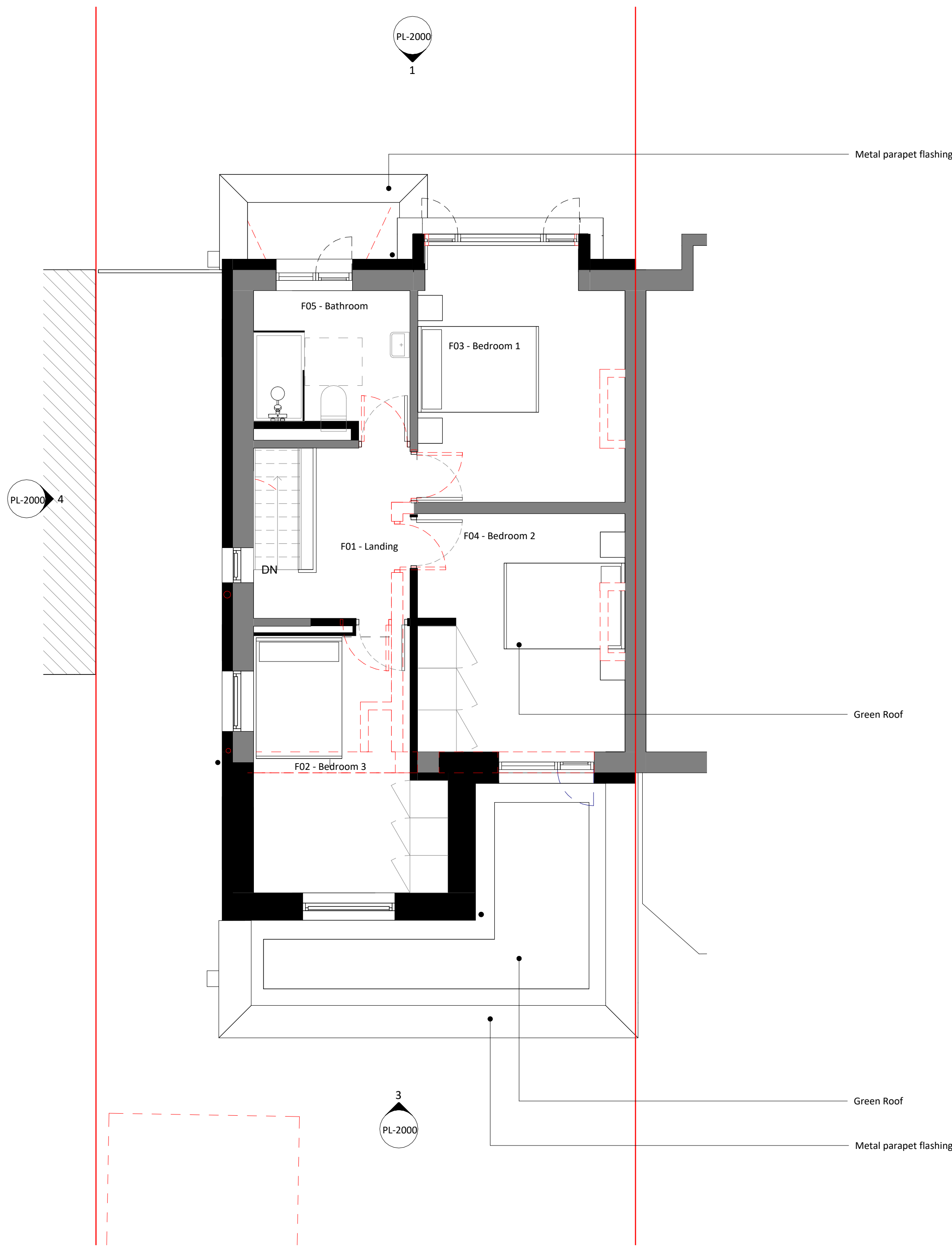
2 Proposed First Floor Plan 1 : 50
