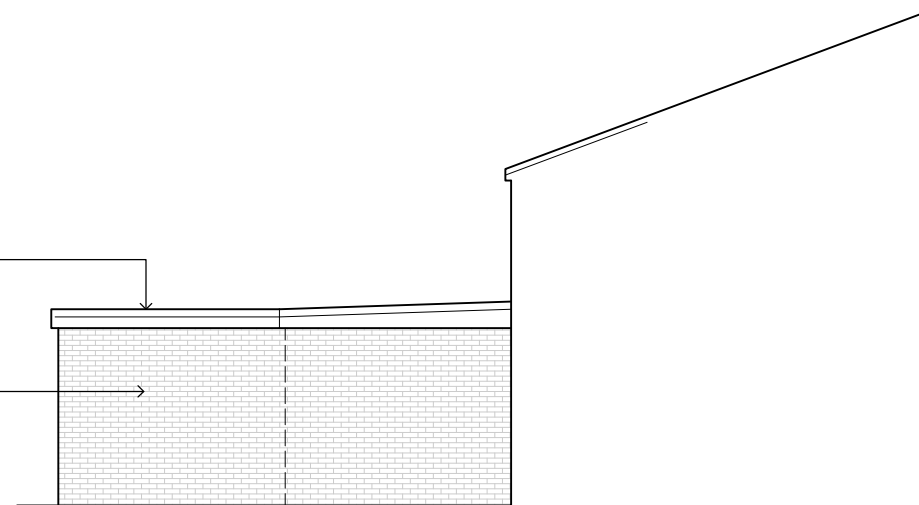
PROPOSED REAR/SIDE ELEVATION 1:100 @ A3
