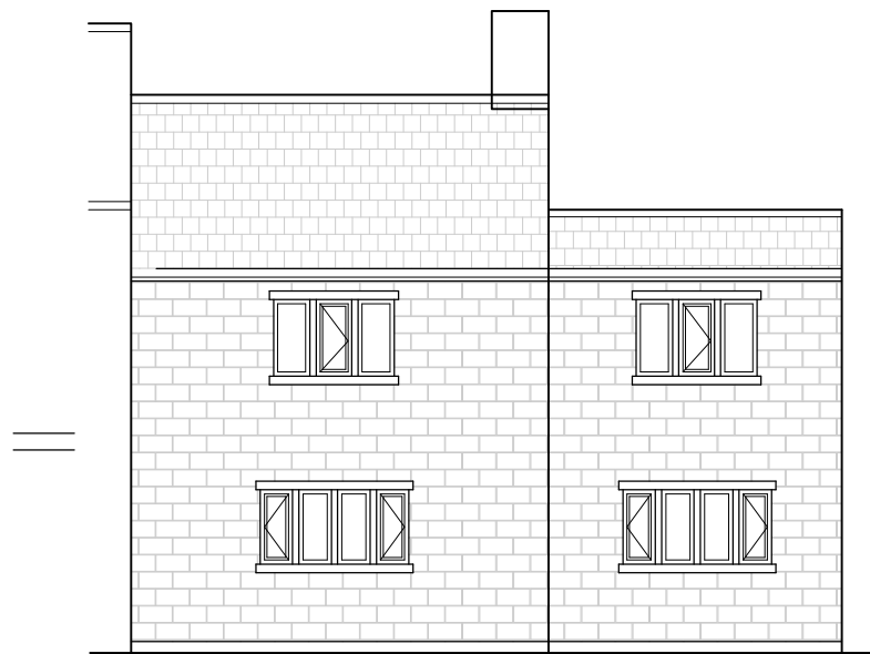
PROPOSED FRONT ELEVATION 1:100 @ A3
