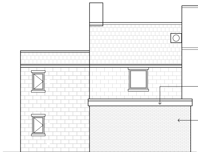
PROPOSED REAR ELEVATION 1:100 @ A3
