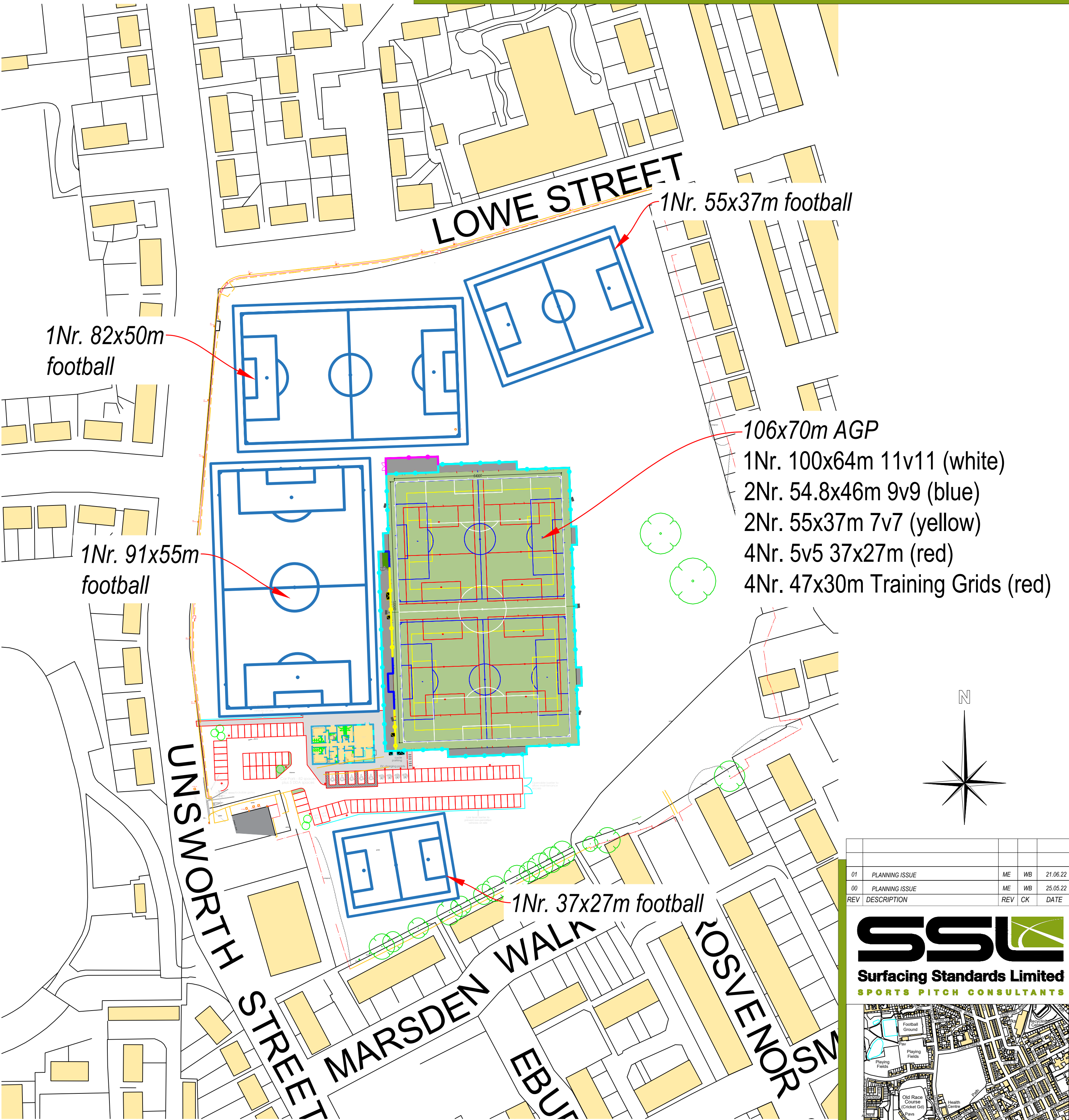
Proposed Playing Field Layout
