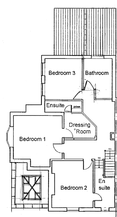
Proposed First
