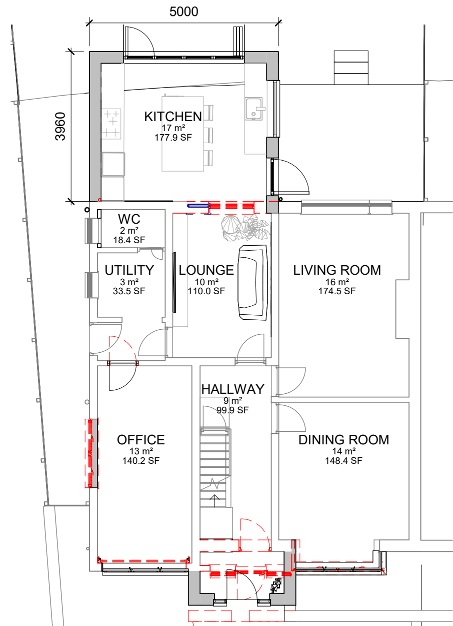
Proposed Ground Floor - Demolitions 1:100
