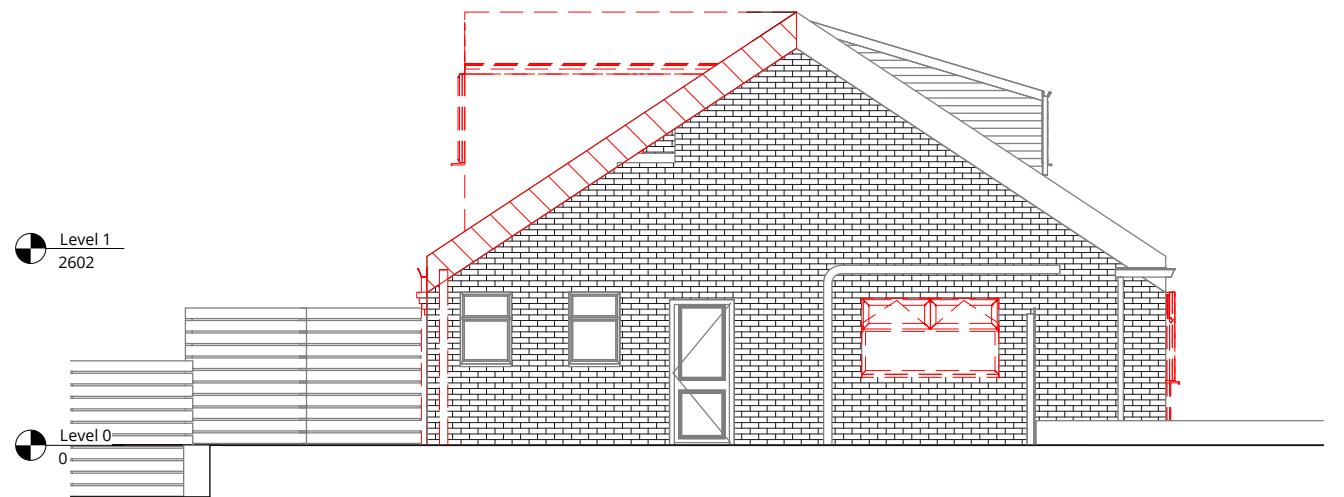
5 Proposed Side Elevation - Demolitions 1:100
