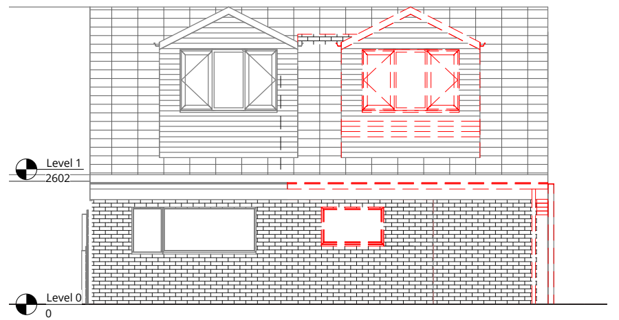
4 Proposed Rear Elevation - Demolitions 1:100
