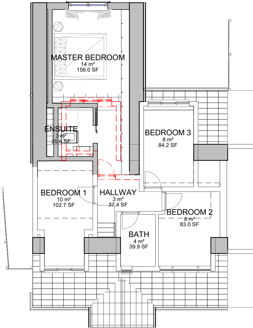
Proposed First Floor - Demolitions 1:100
