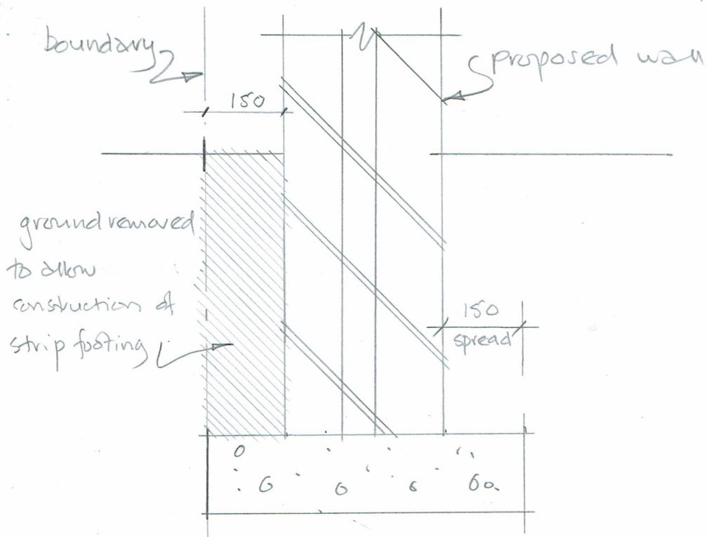
CONVENTIONAL STRIP FOOTING
