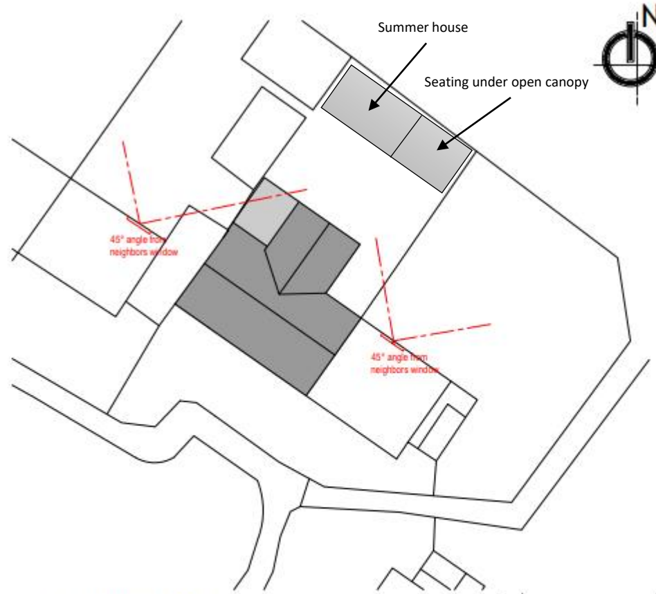
Block Plan 1:200
