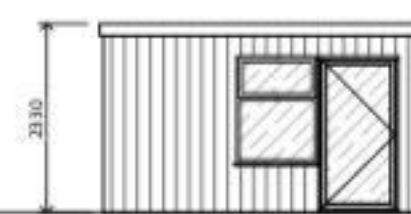
Rear Elevation Scale 1:50 @ A1 1:100 @ A3
