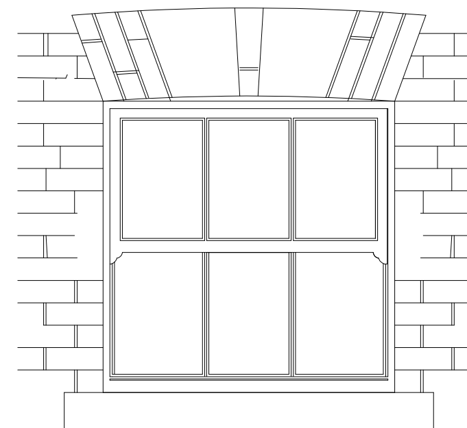
New windows to locate into same position within masonry aperture as existing
