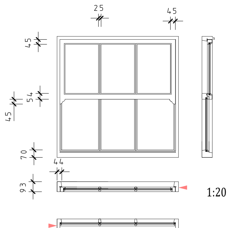
Proposed replacement windows to The Stables, Prestwich, M250NH
