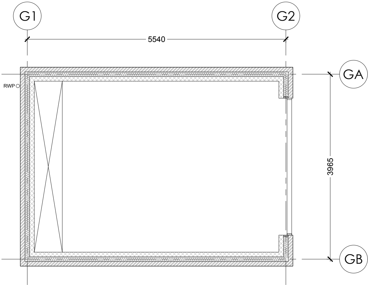
DETACHED GARAGE, PROPOSED PLAN 1:50
