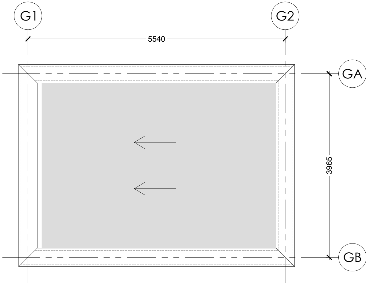
DETACHED GARAGE, PROPOSED ROOF PLAN 1:50
