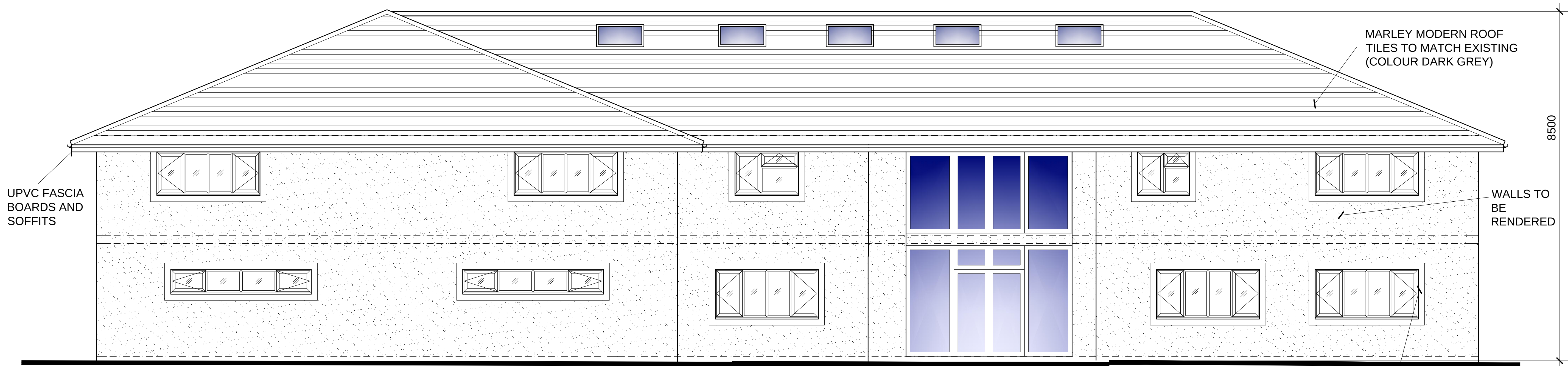
PROPOSED FRONT (Balcony not shown)
