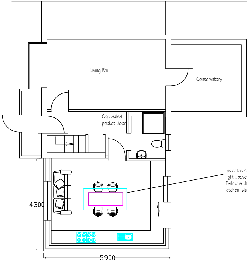
Proposed Plan
