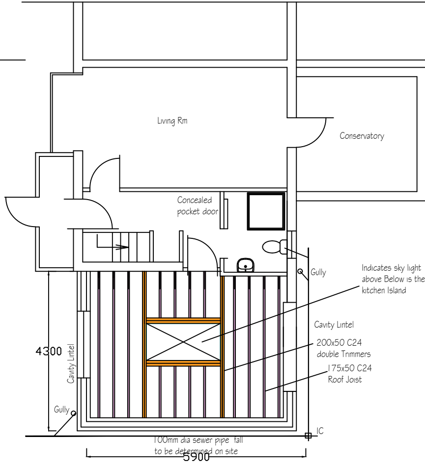
Proposed Plan
