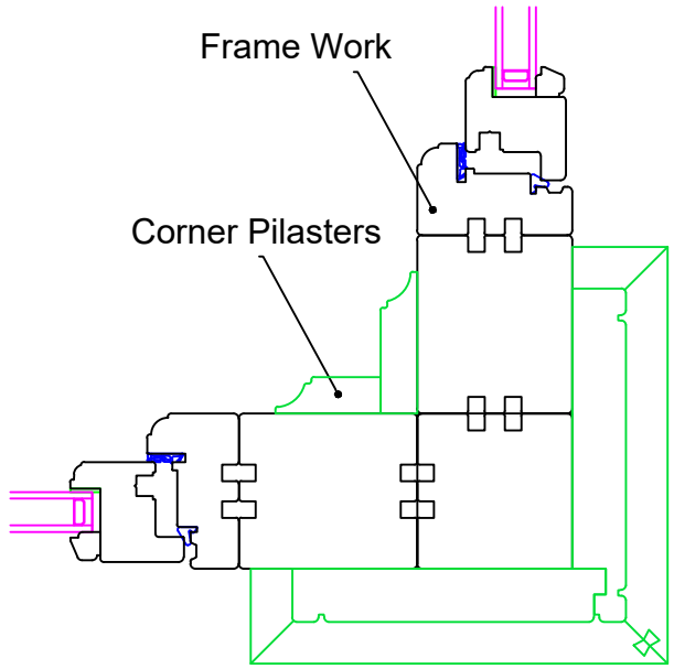
PLAN VIEW OF CORNER PILASTERS Scale 1:5
