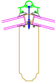
Hip Detail
