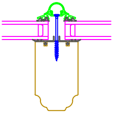
Rafter Detail
