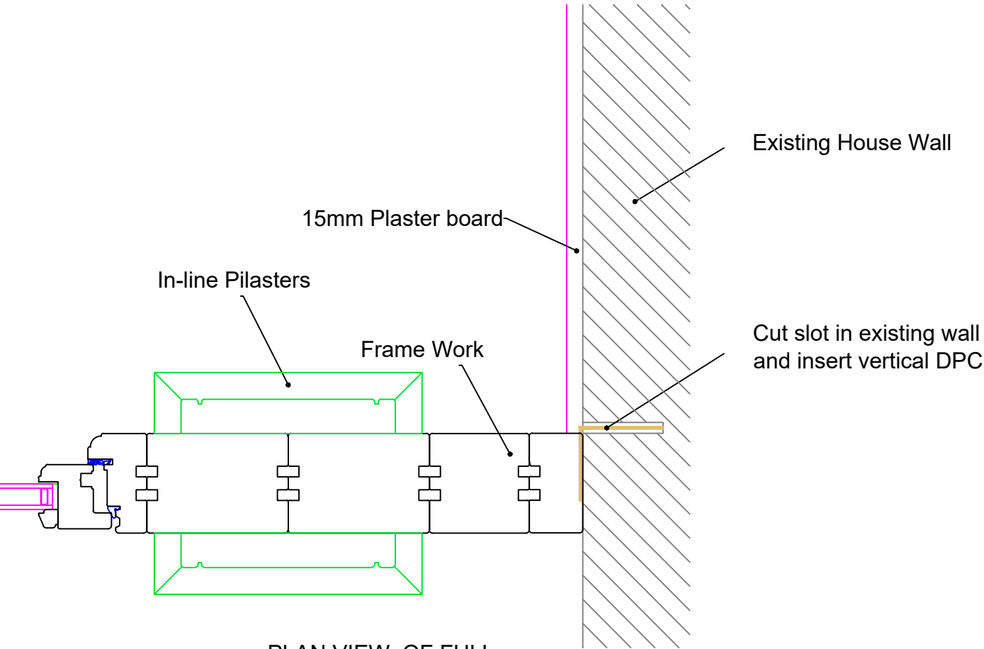
PLAN VIEW OF FULL HEIGHT FRAME AT WALL Scale 1:5
