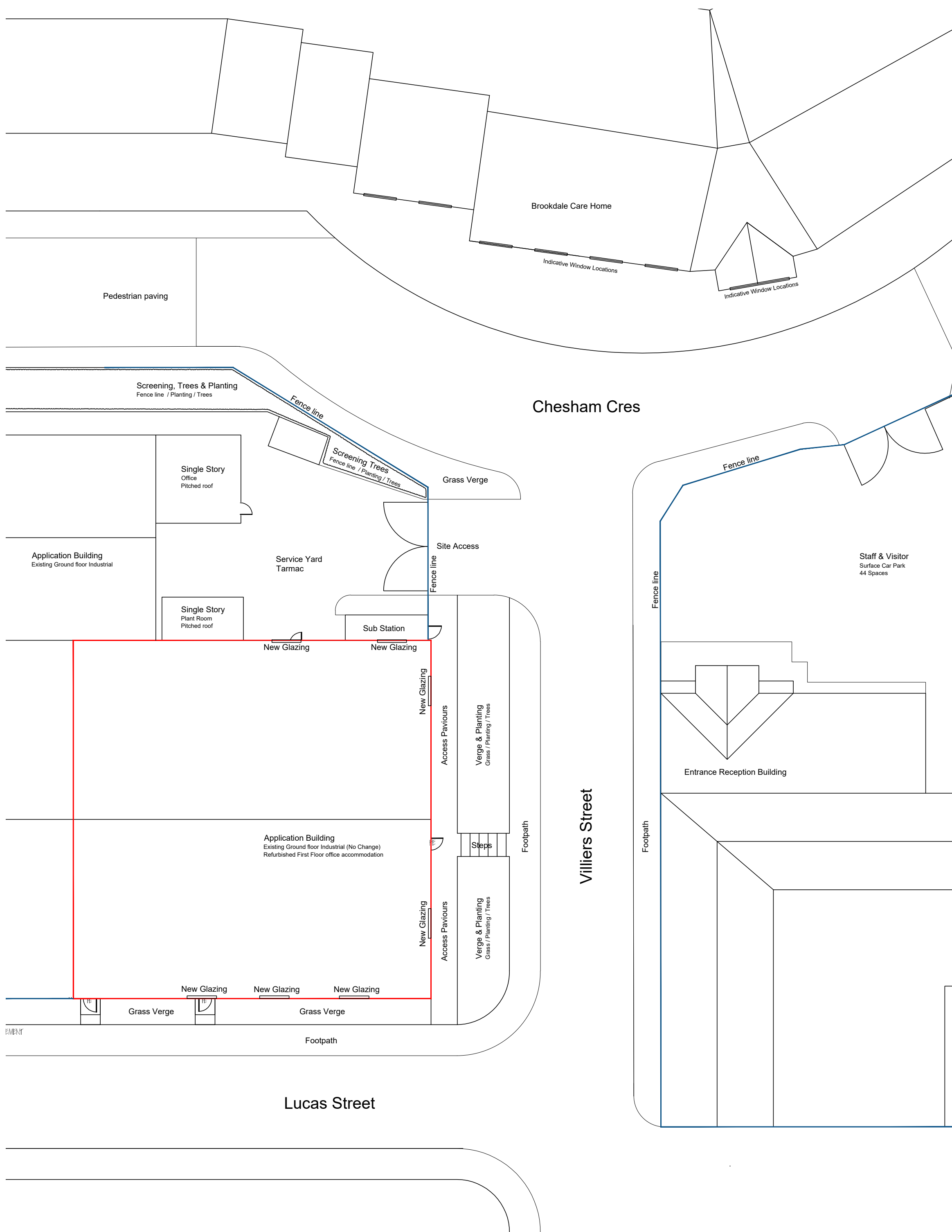
2 Proposed Site Layout plan 1 : 200
