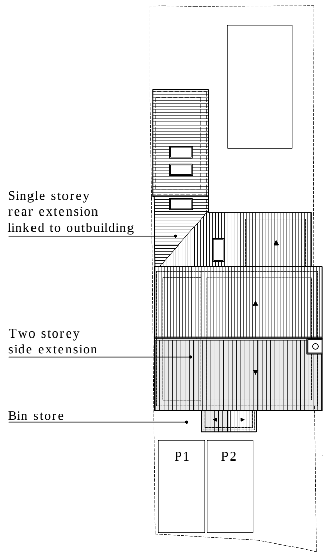
Proposed site / roof plan 1:200
