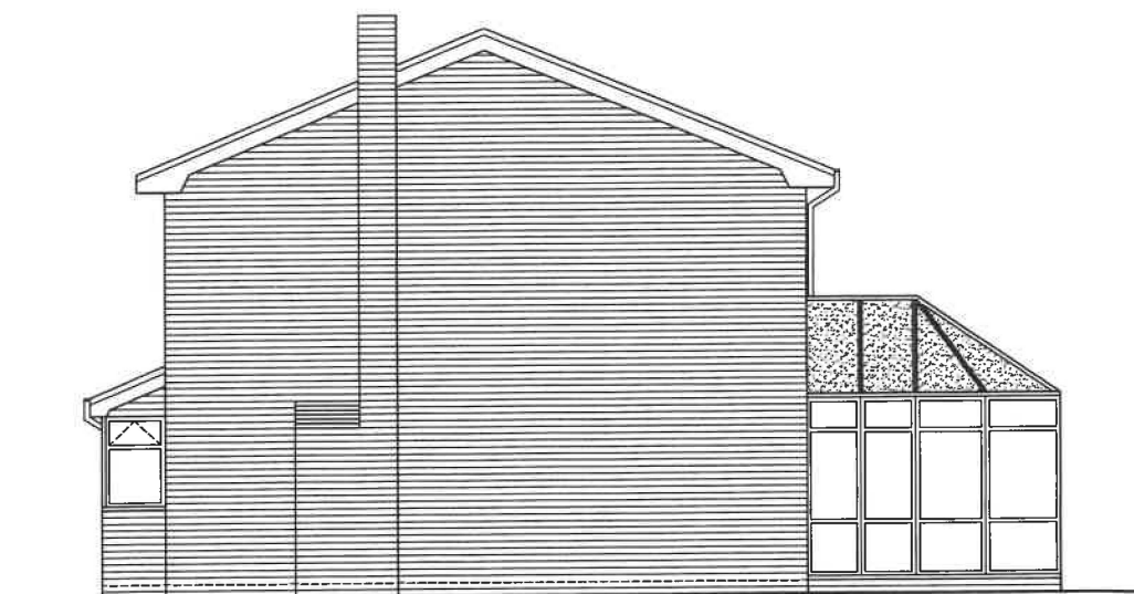
EXISTING SIDE ELEVATION [AS VIEWED FROM NO.6] 1:100 @ A4
