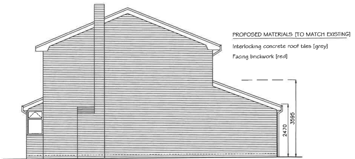
PROPOSED SIDE ELEVATION [AS VIEWED FROM NO.6] 1:100 @ A4
