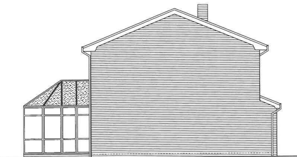
EXISTING SIDE ELEVATION [AS VIEWED FROM NO. 10] 1:100 @ A4
