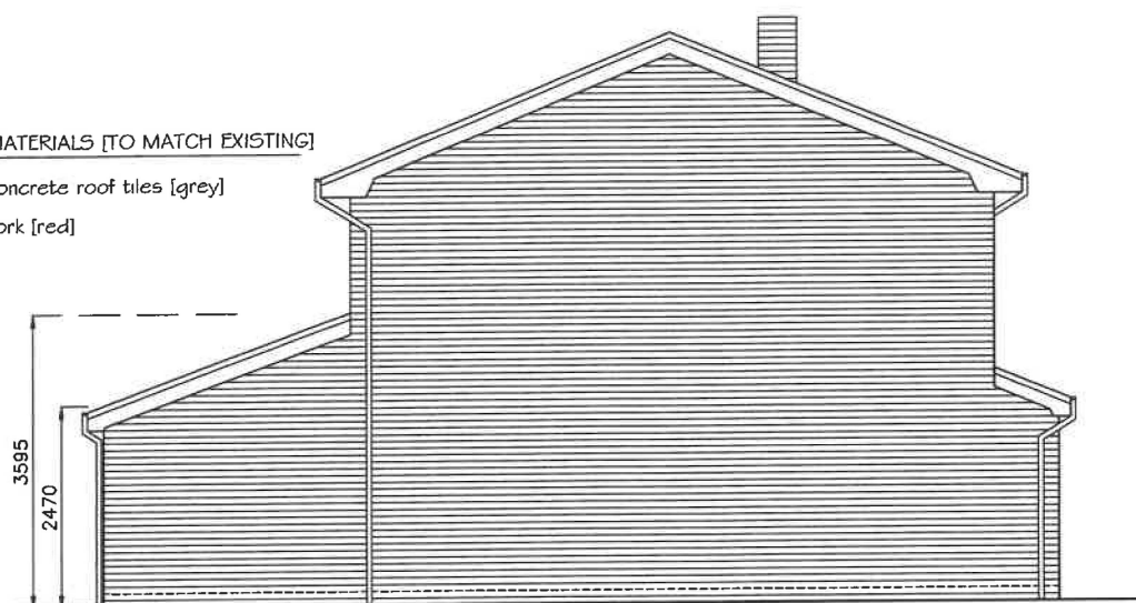
PROPOSED SIDE ELEVATION [AS VIEWED FROM NO. 10] 1:100 @ A4
