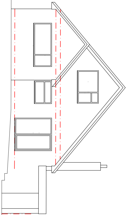
REAR ELEVATION 1:100
