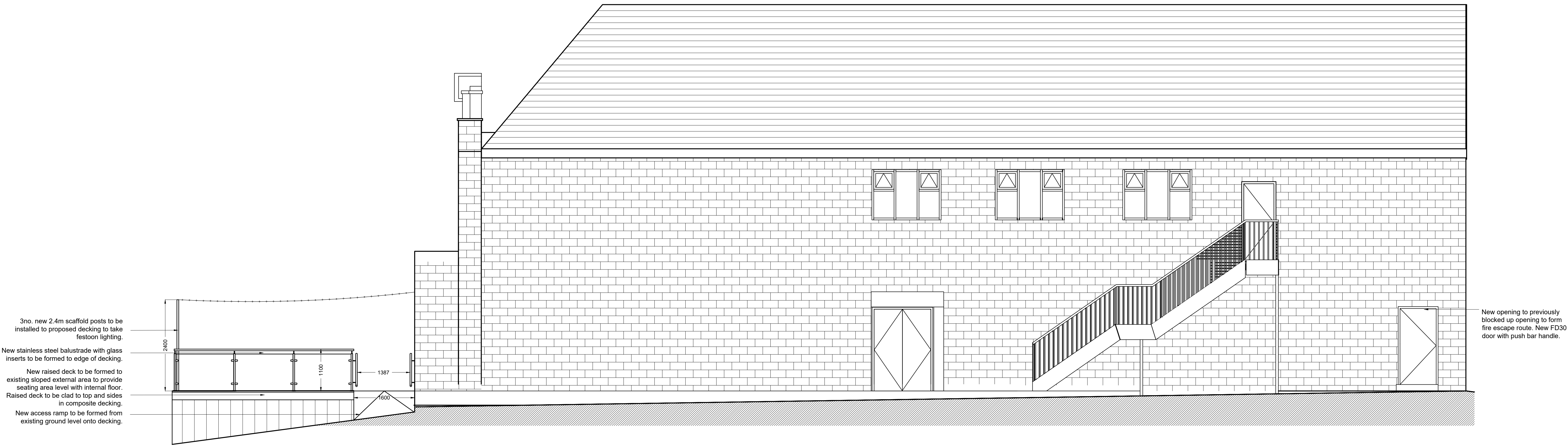
PROPOSED SIDE ELEVATION Scale 1:50
