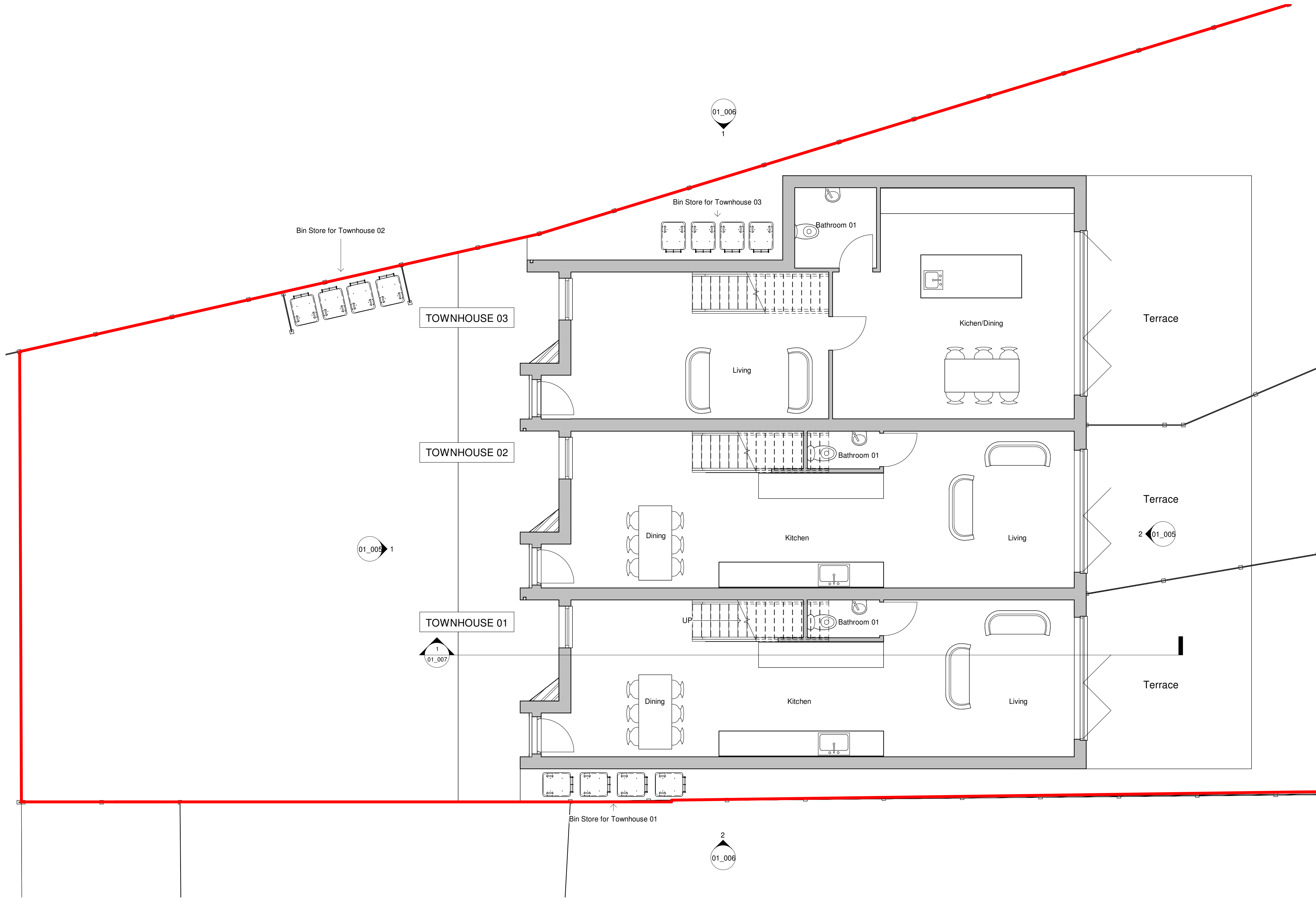
00 Proposed Ground Floor 1 : 50
