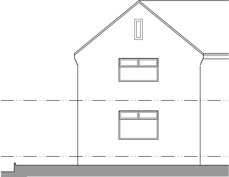
North Facing Front Elevation
