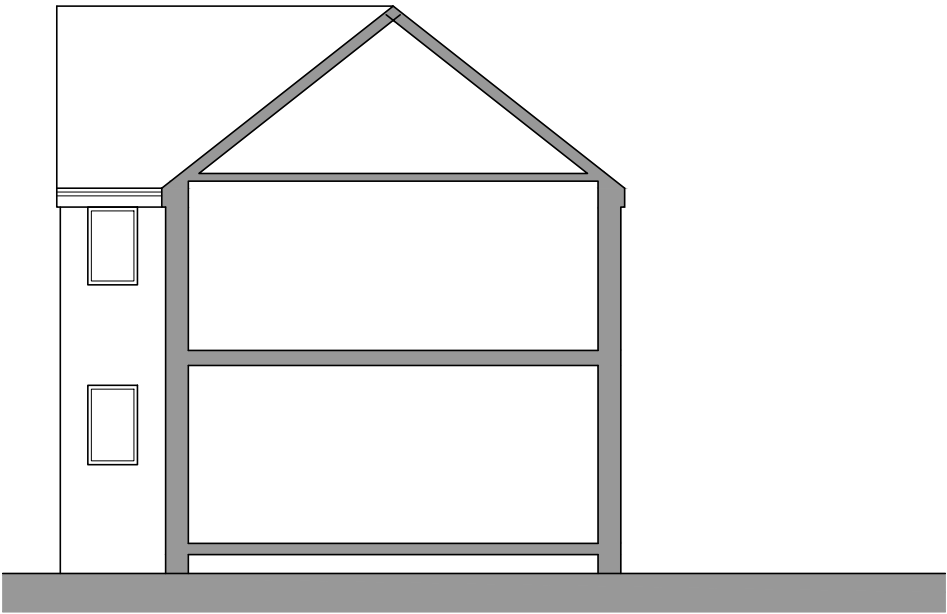
West Facing Side Elevation
