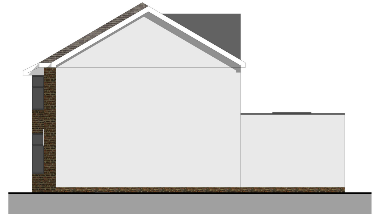
proposed side elevation 1 scale 1:100
