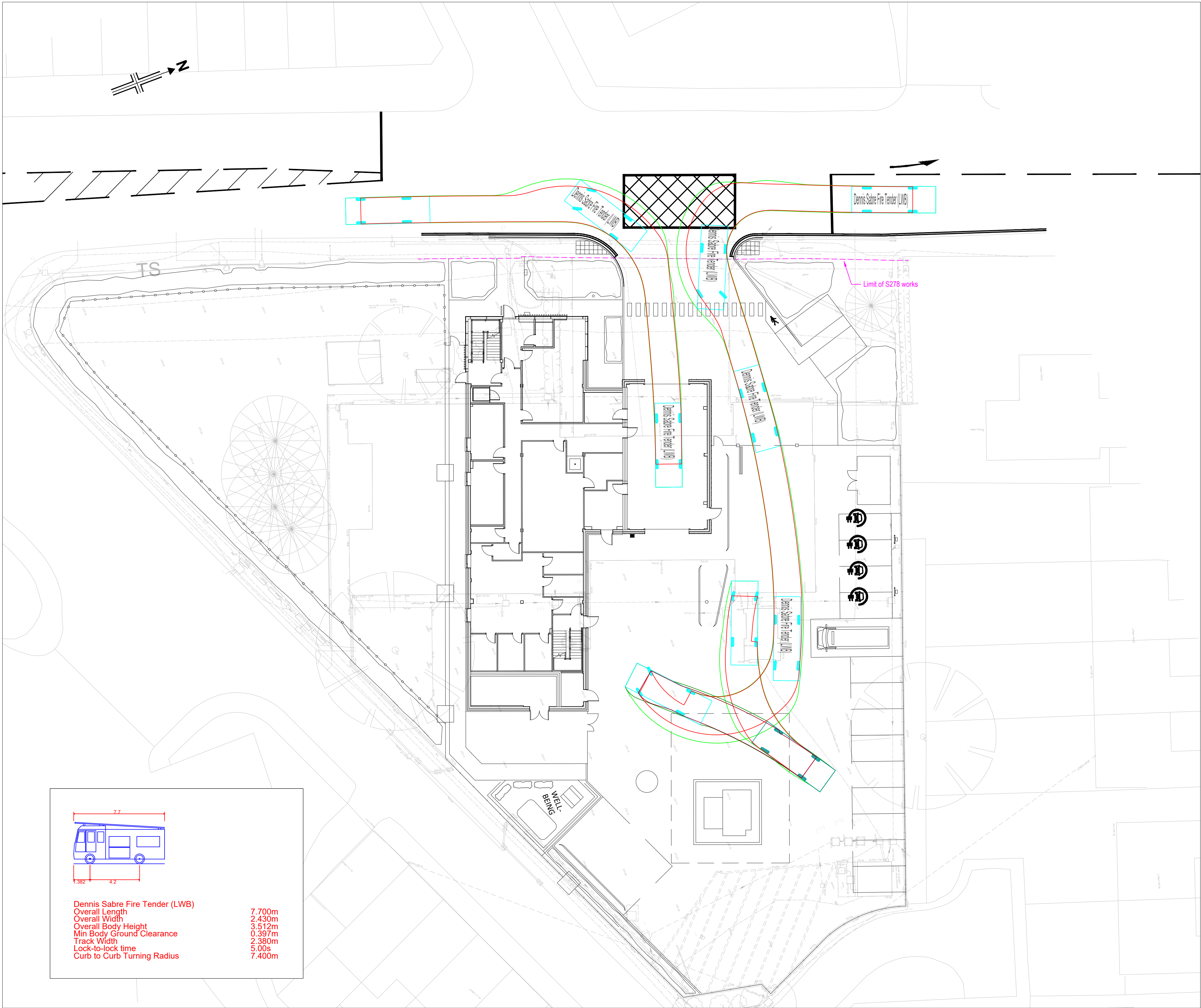
Swept Path - LWB Fire Tender (Scale 1:200)
