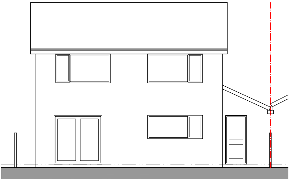
East Facing Rear Elevation
