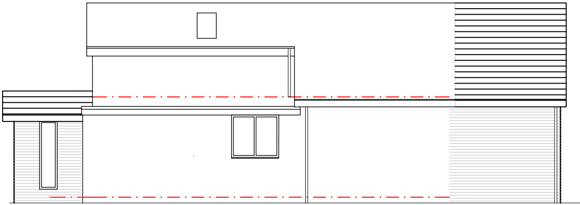
SIDE ELEVATION 1:100
