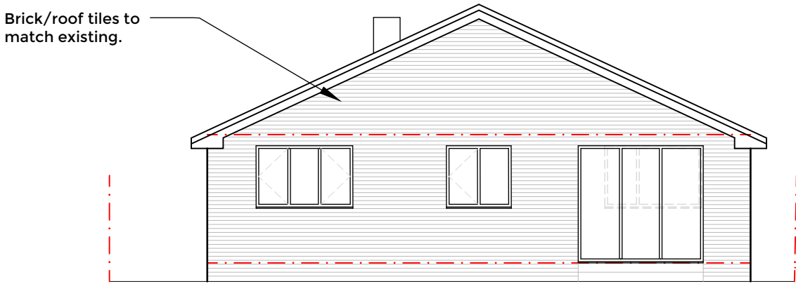
REAR ELEVATION 1:100
