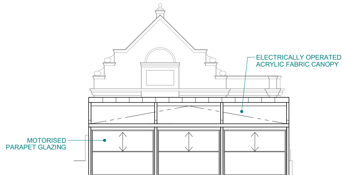
PART SOUTH ELEVATION
