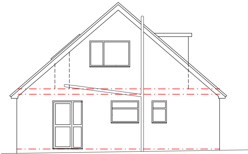
SIDE ELEVATION 1:100
