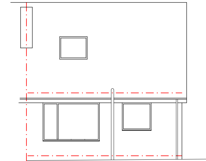
REAR ELEVATION 1:100
