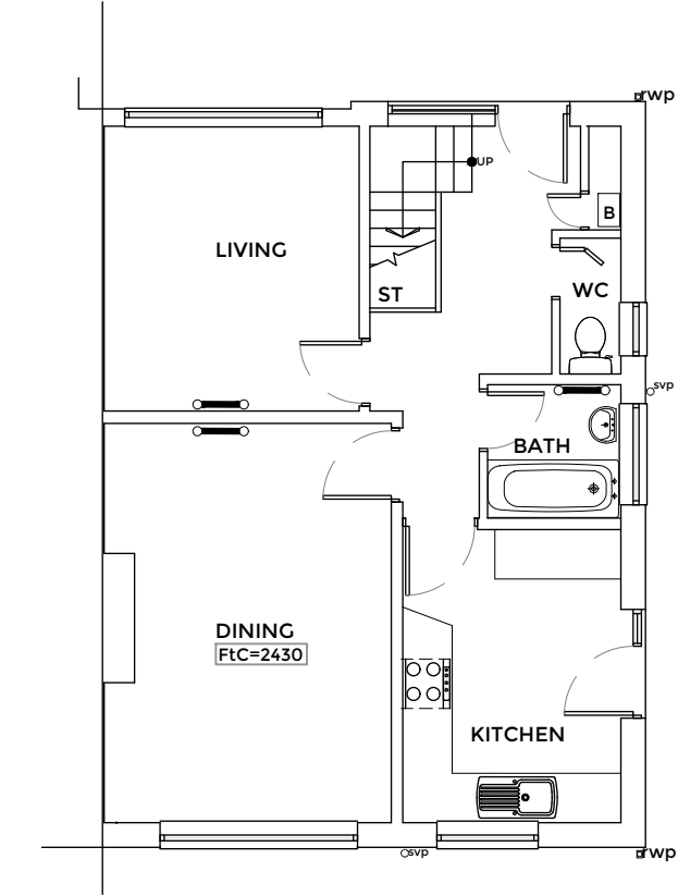
GROUND FLOOR PLAN 1:100 Walls to be checked for load bearing.
