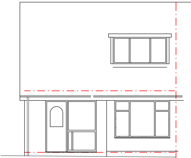
FRONT ELEVATION 1:100
