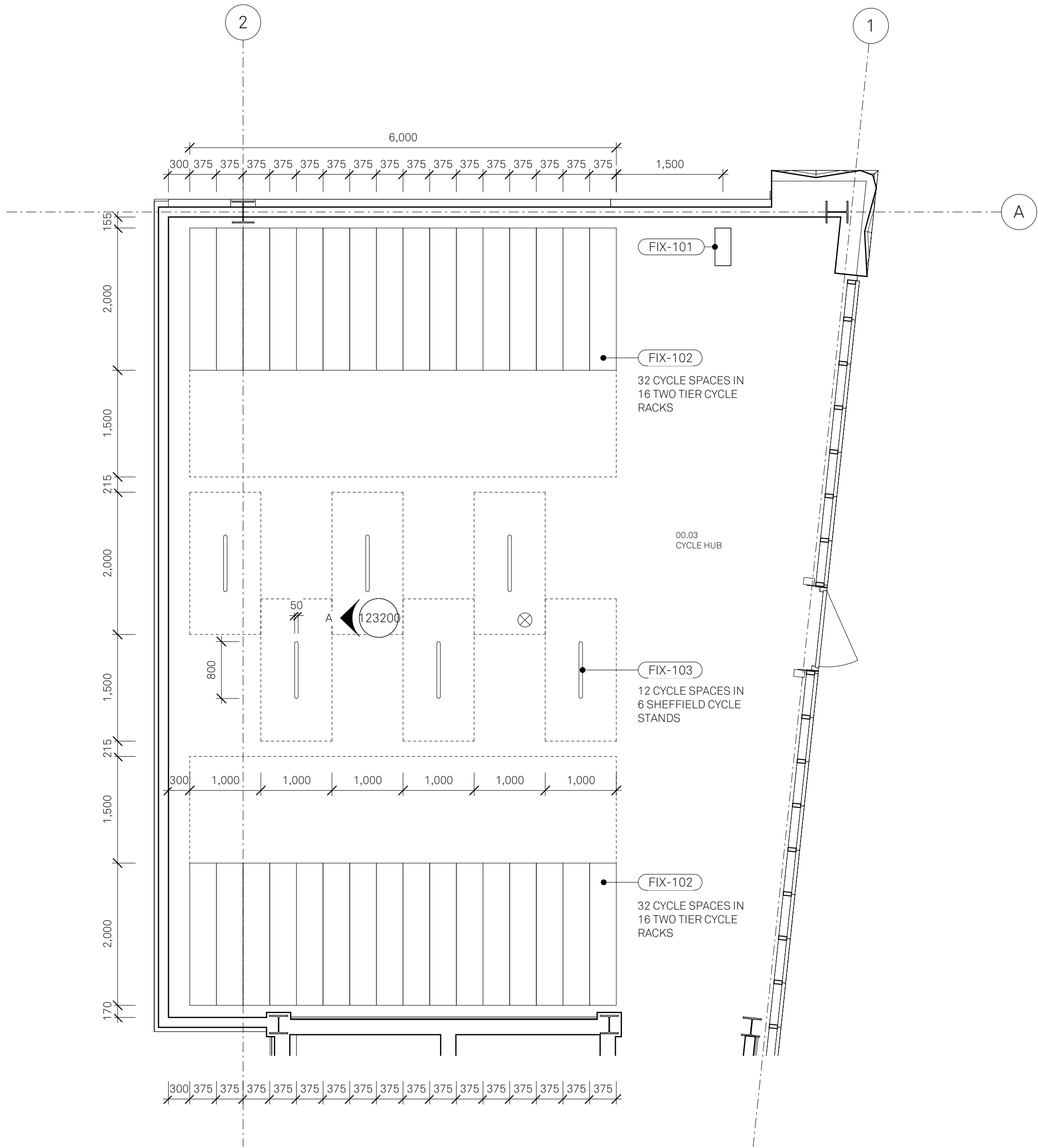
CYCLE HUB SETTING OUT PLAN 76 TOTAL CYCLE SPACES
