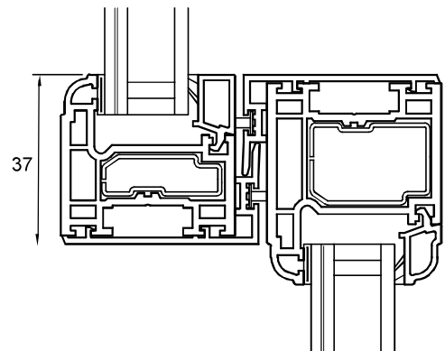
Meeting Rail
