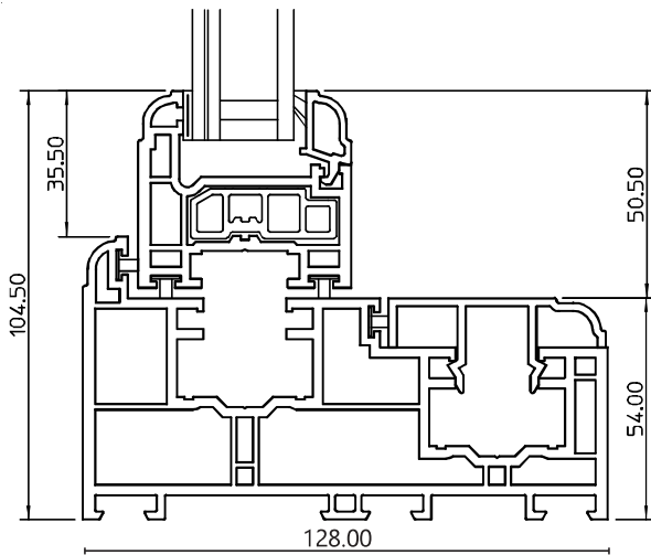
Top Rail
