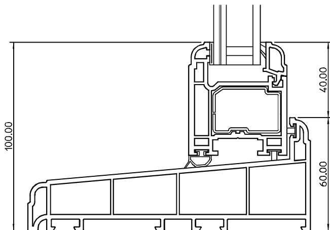
Bottom Rail
