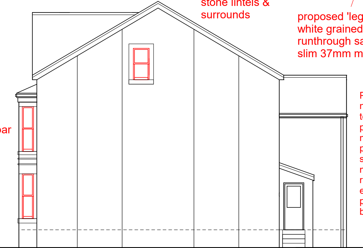
right side (southwest) elevation
