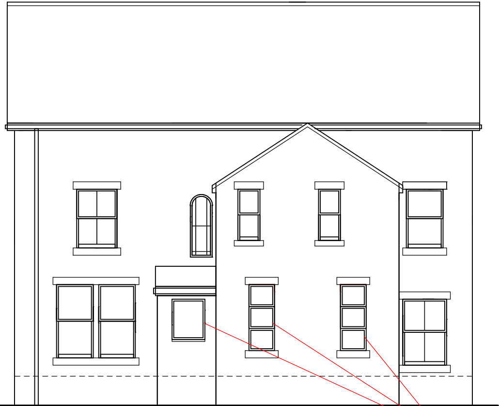
rear (southeast) elevation
