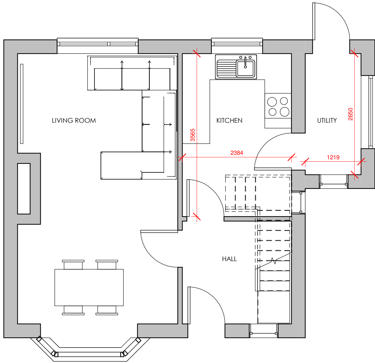
01 EXISTING GROUND FLOOR 1 : 50
