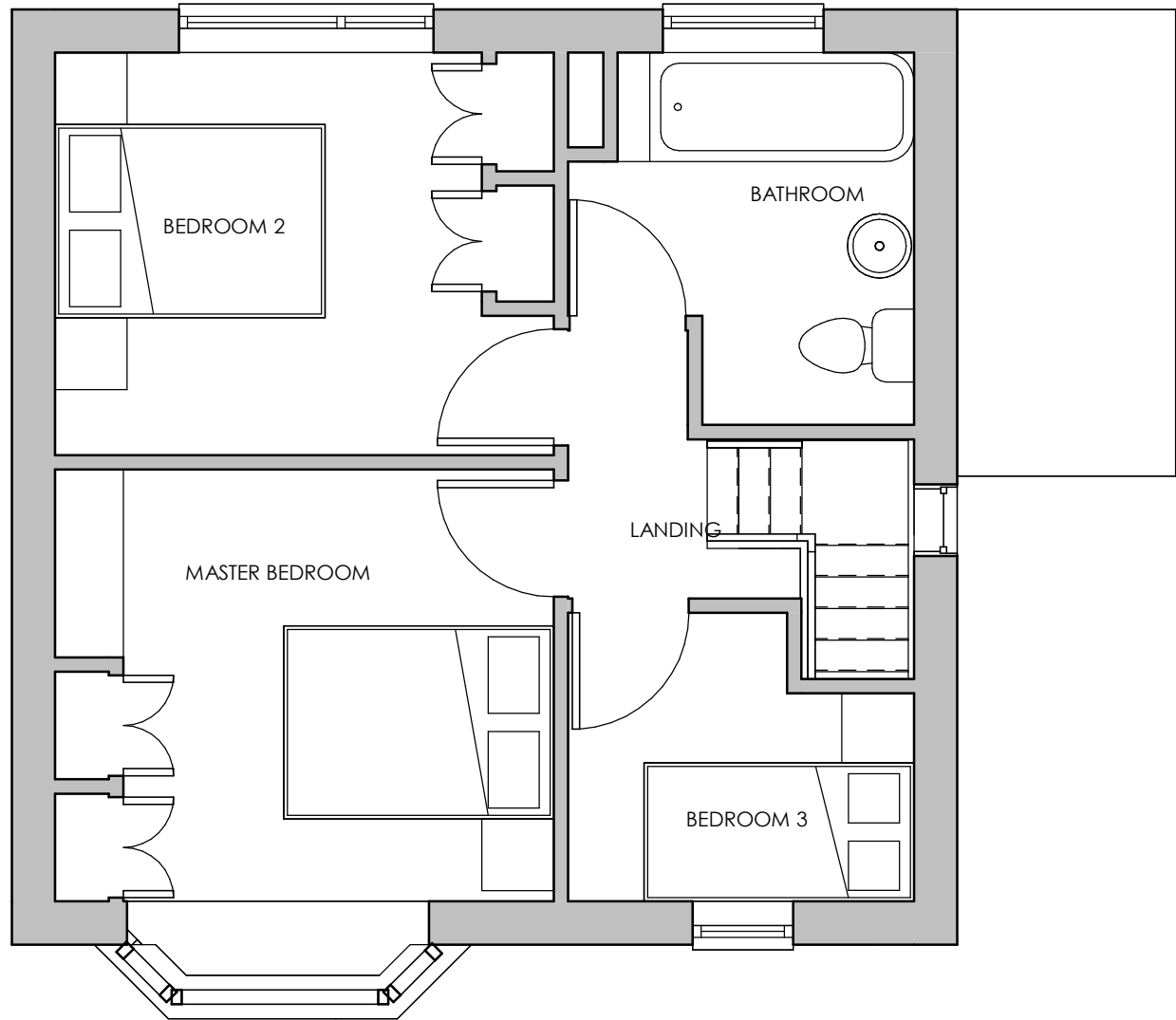
02 EXISTING FIRST FLOOR 1 : 50
