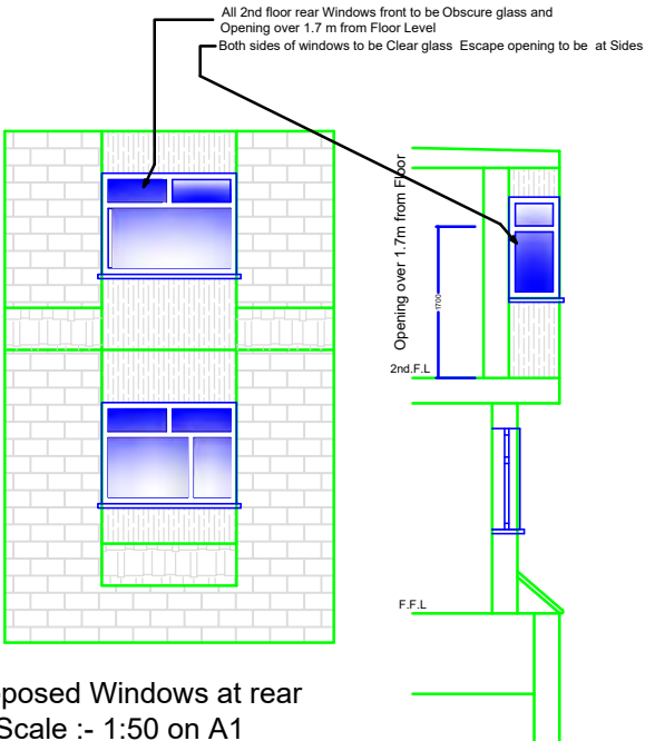
Proposed rear Windows Side Elevation @ Scale :- 1:50 on A1
