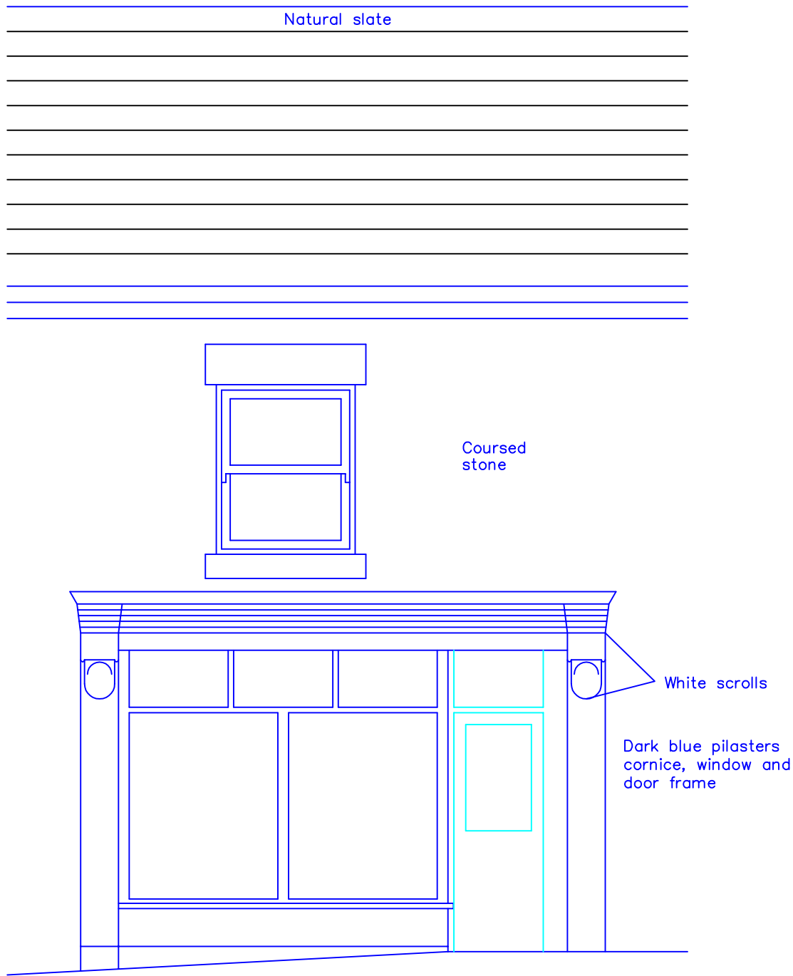
Original Front Elevation
