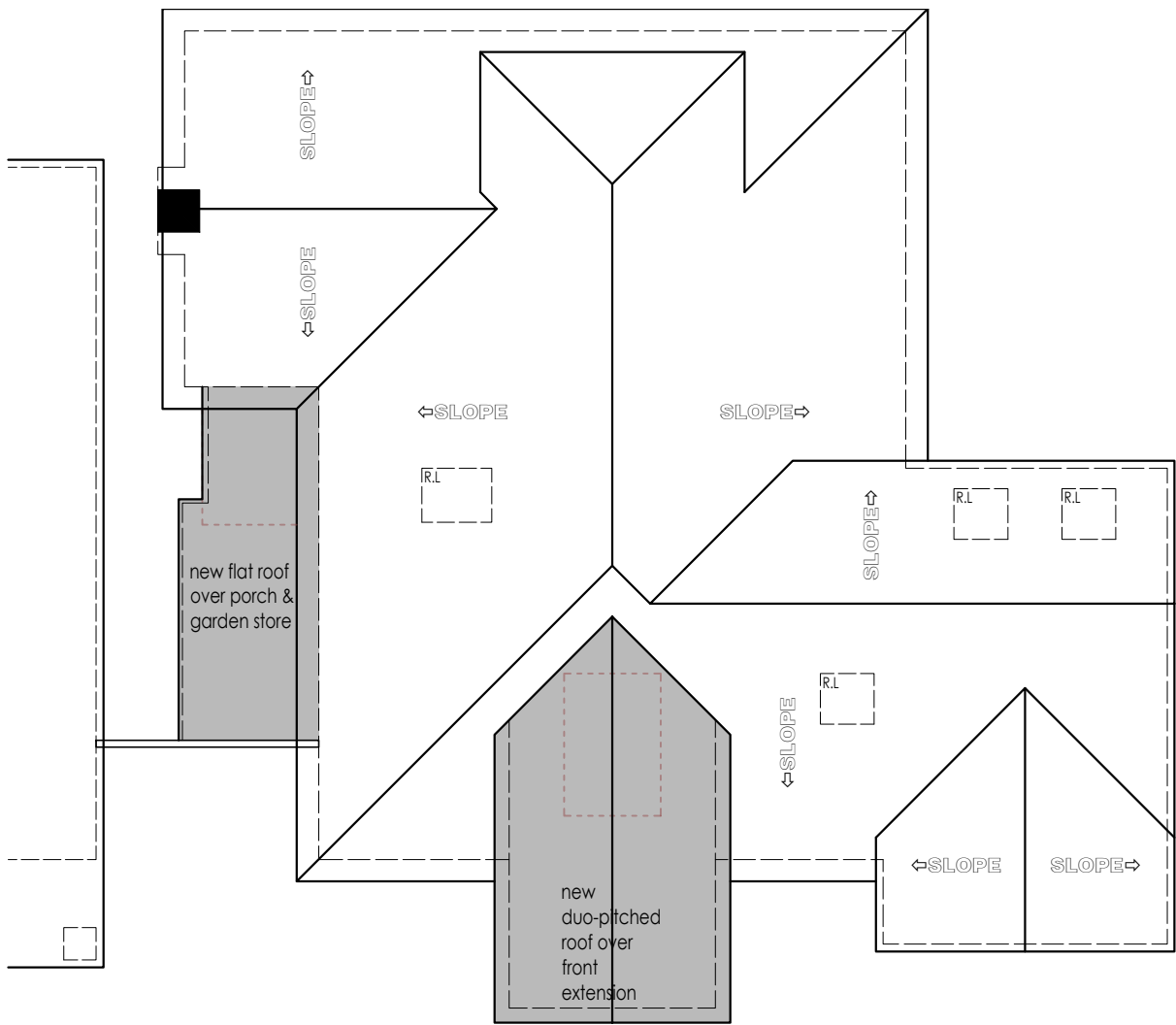
ROOF PLAN
