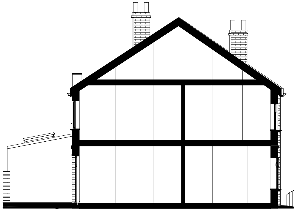
6 Existing Side Elevation Through No. 42 1 : 100
