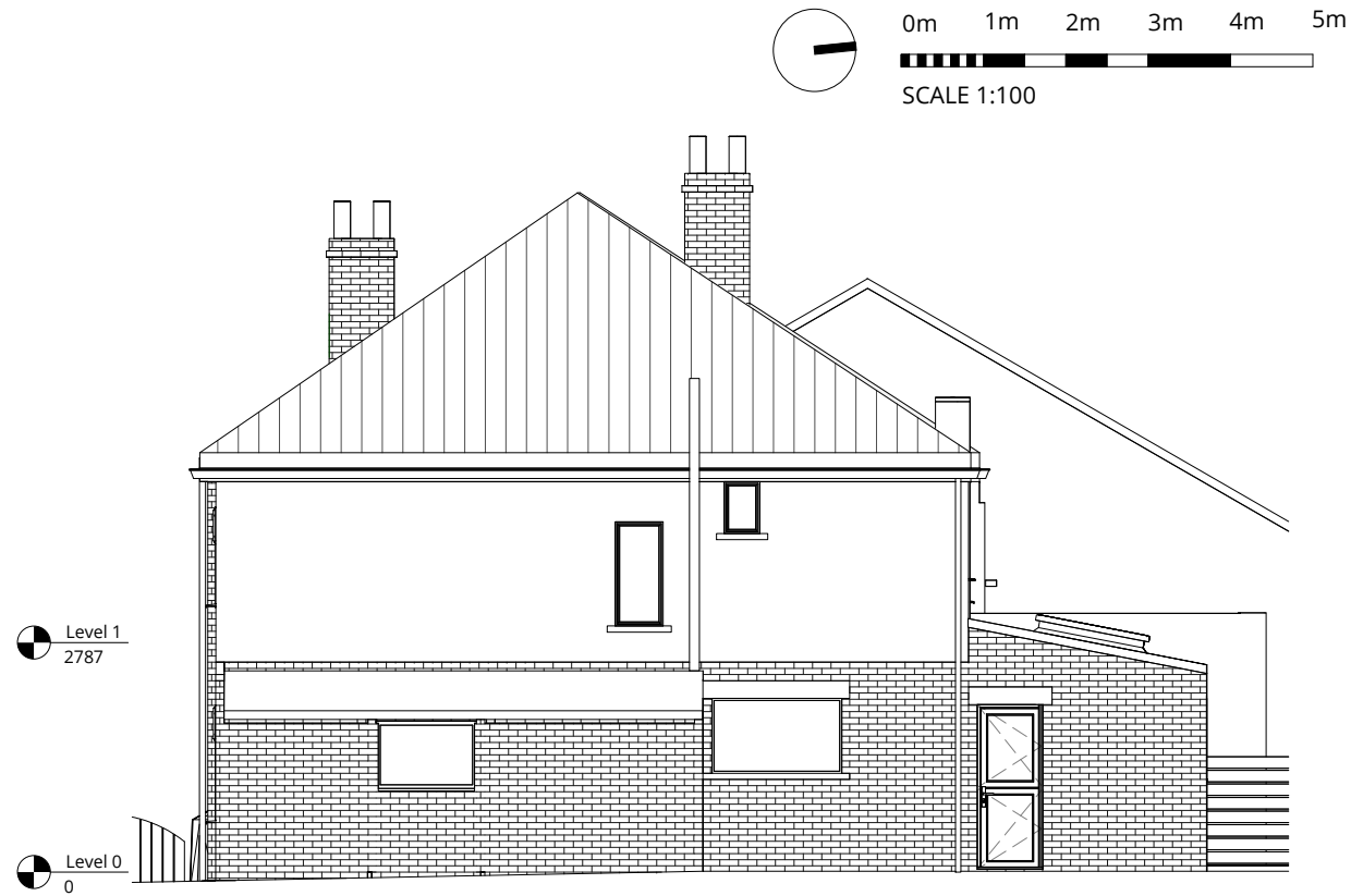
5 Existing Side Elevation 1 : 100
