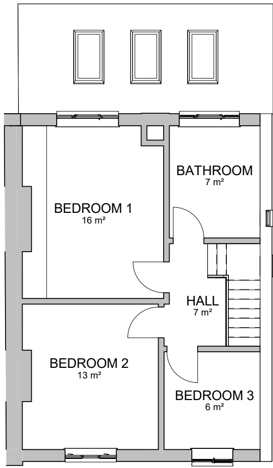
2 Existing First Floor Plan 1 : 100
