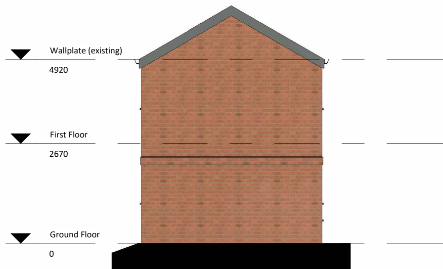
11 Rear Proposed 1 : 100
