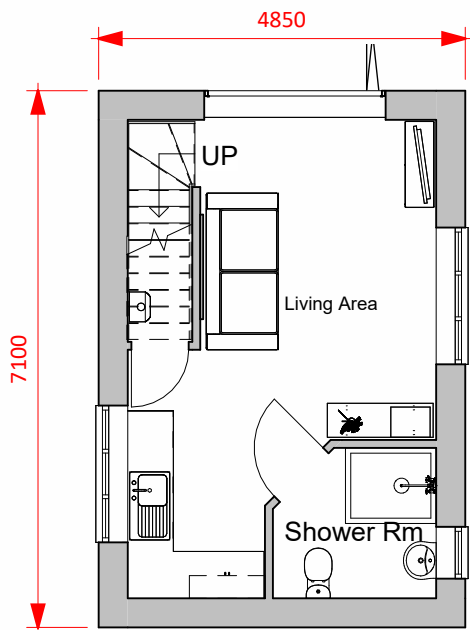
02b GF Proposed 1 : 100
