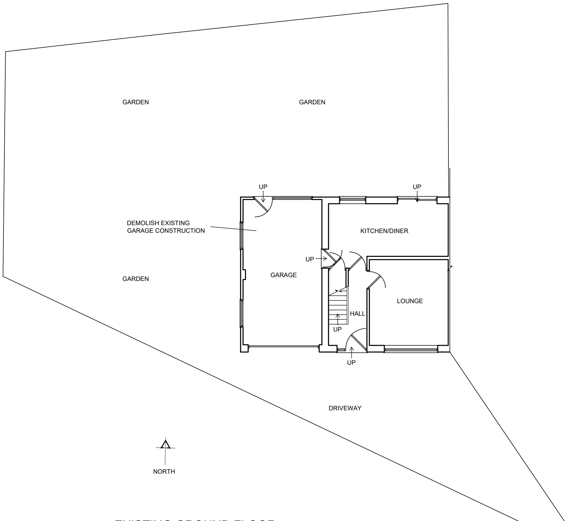
EXISTING GROUND FLOOR & SITE LAYOUT @ 1 : 100
