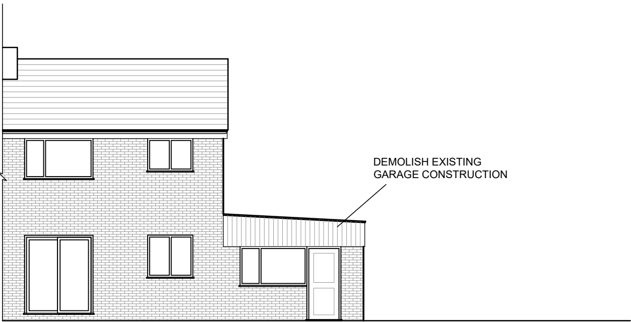
EXISTING NORTH FACING ELEVATION @ 1 : 100
