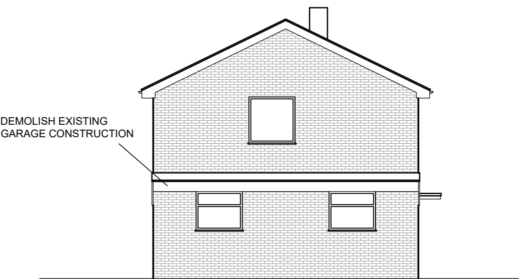
EXISTING WEST FACING ELEVATION @ 1 : 100
