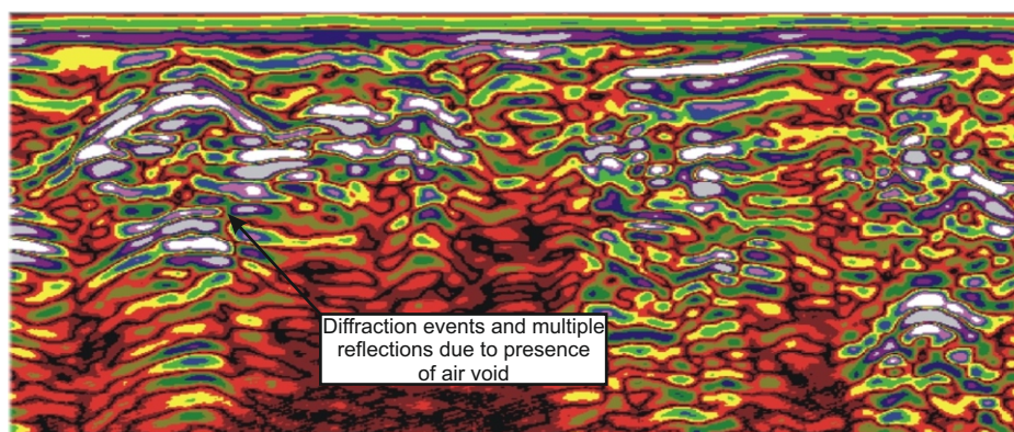
C An example of mid frequency (400MHz) radar data collected over a voided grave
