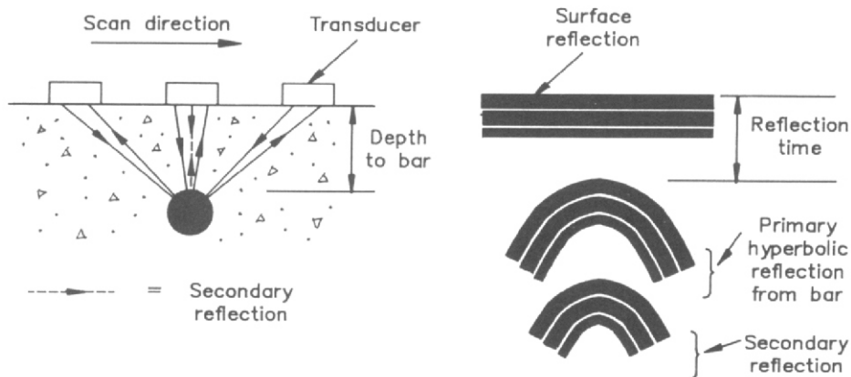
B GPR response to rebar or service
