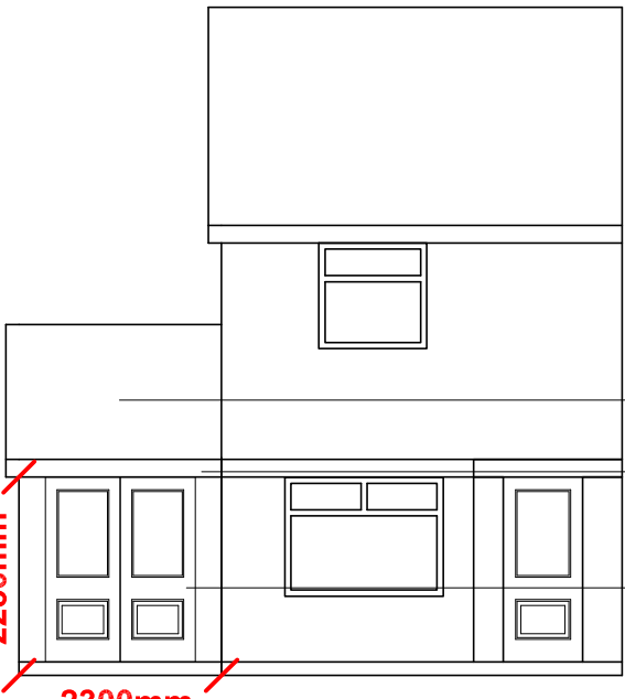
PROPOSED SIDE EVATION 1:100
