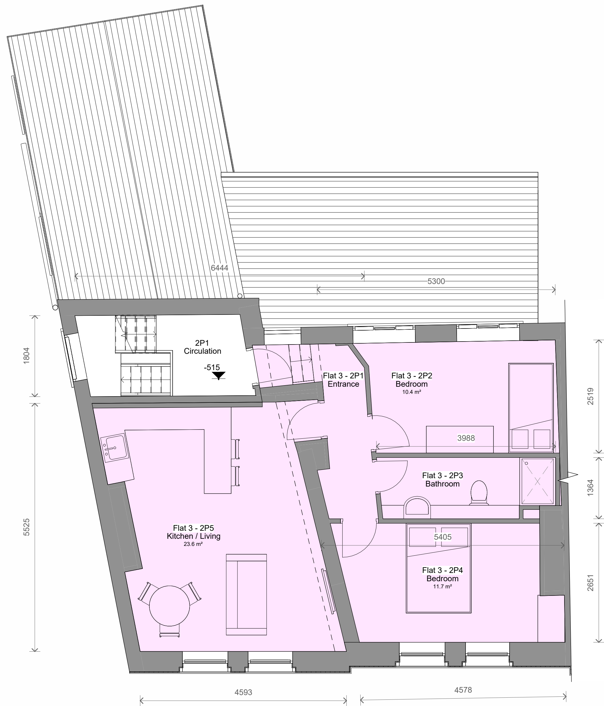
1 Level 2 - Proposed 1 : 50
