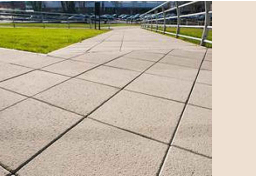
Buff flagged patios / paths Buff 450 x 450mm flags on course sand & compacted ground
