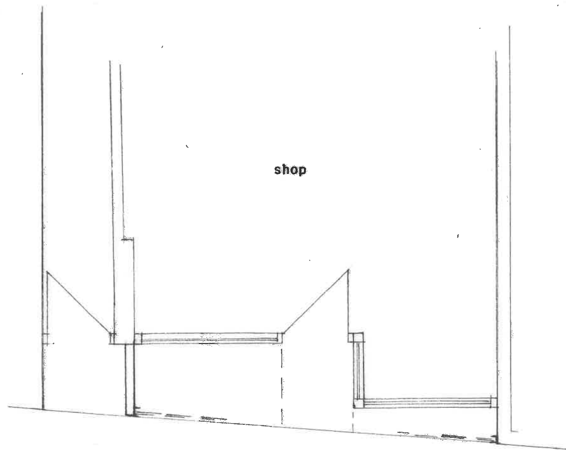
G.F. PLAN (PROPOSED)
