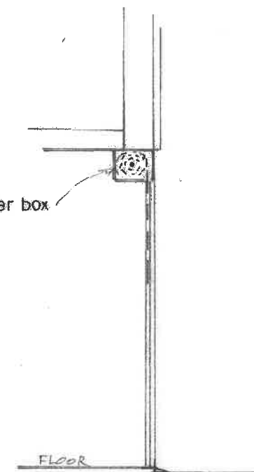
SECTION (PROPOSED)
