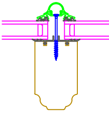
Rafter Detail
