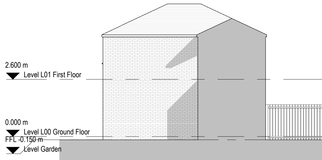
4 Existing North Elevation 1 : 100
